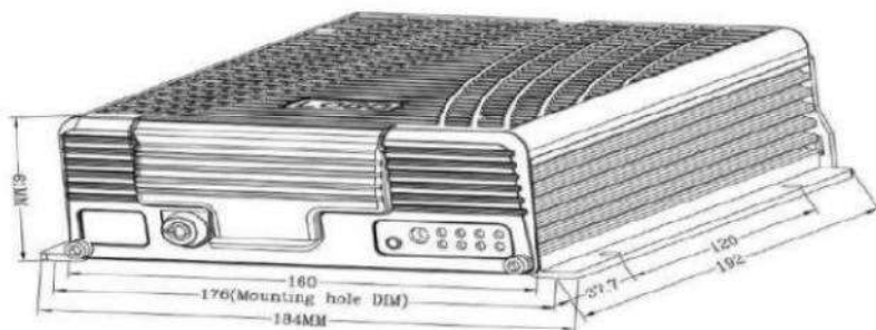
General Dimensions
